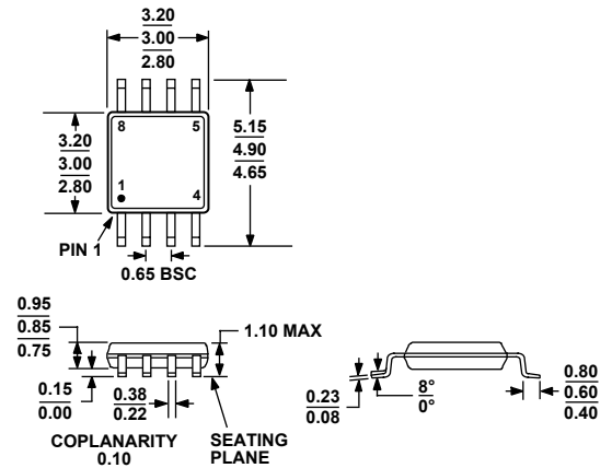
Figure 85. 8-Lead Mini Small Outline Package [MSOP] (RM-8)
